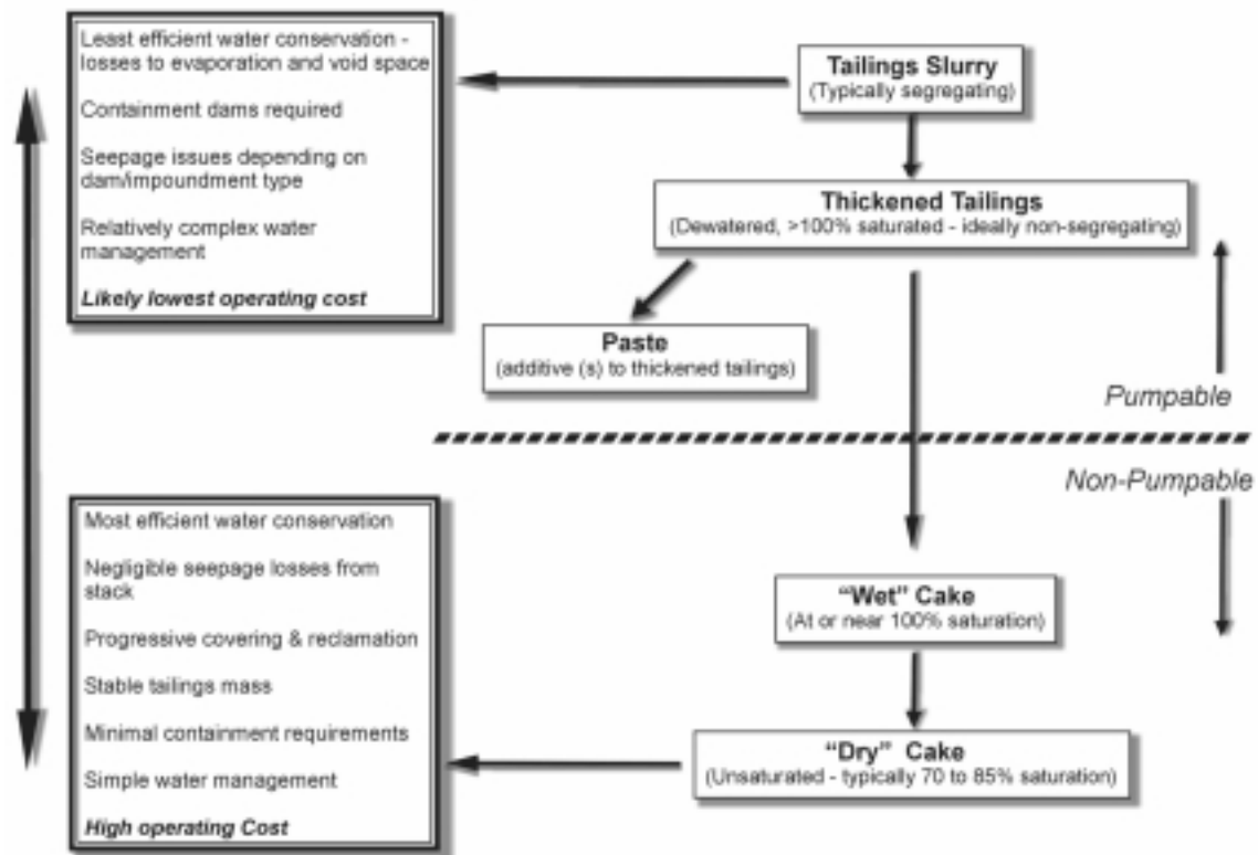
Figure 9. Classification of tailings by degree of dewatering
