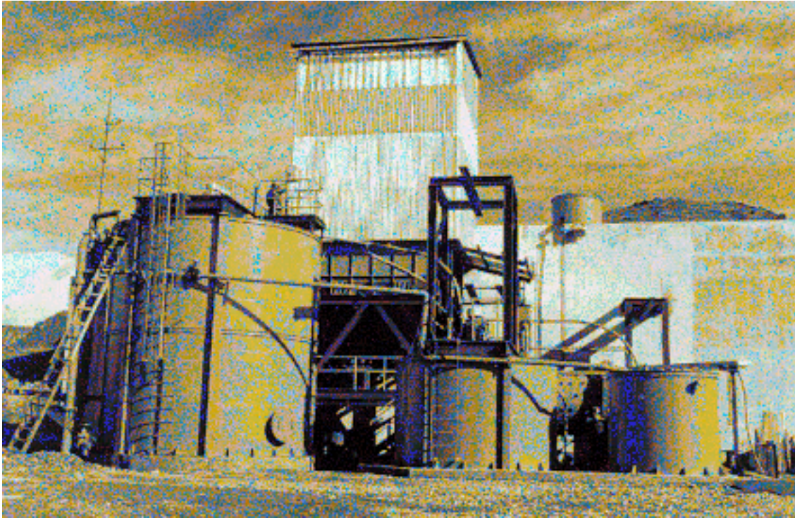
Figure 13 Lime treatment plant for neutralizing acidic mine drainage
